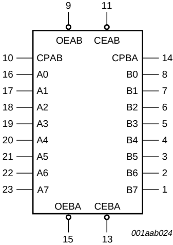
Fig 2. Logic symbol.
